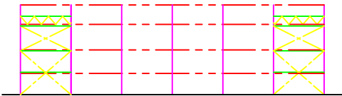
ELEVATION B-B; INNER BOOM 76x76 x9.5RSA SIDE PURLINS JOINTED @ 3810 CTRS
