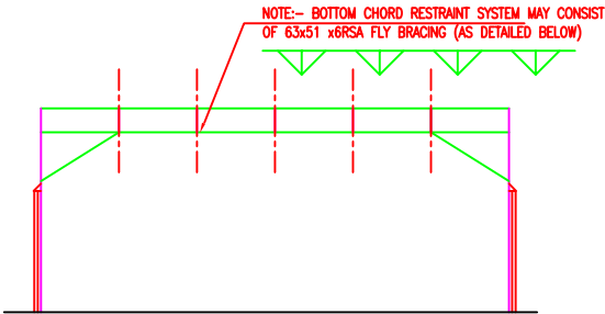
TYPICAL SECTION A-A
