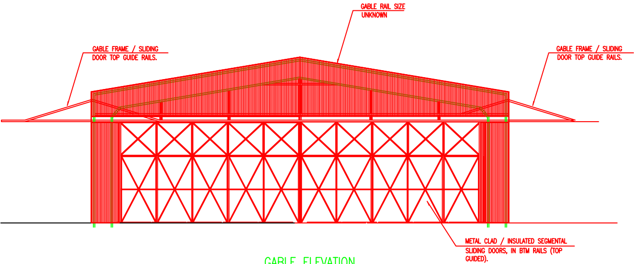
GABLE ELEVATION
