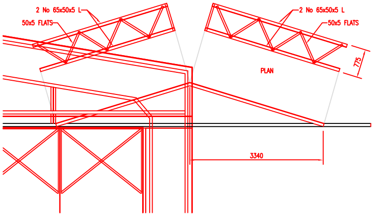
TYPICAL DOOR TRACK SUSPENDER DETAIL
